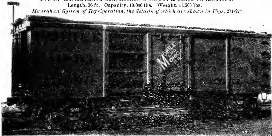
Fig. 11. REFRIGERATOR CAR, MOBILE & OHIO RAILROAD. Capacity, 40,000 lbs. Weight, 37,400 lbs.
